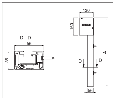
VS6200 Wall mounting with direct screw connection
